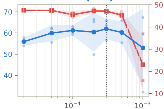
SC-LoRA
