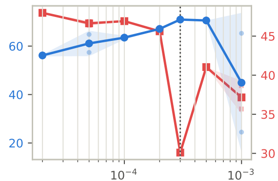
CLoRA
